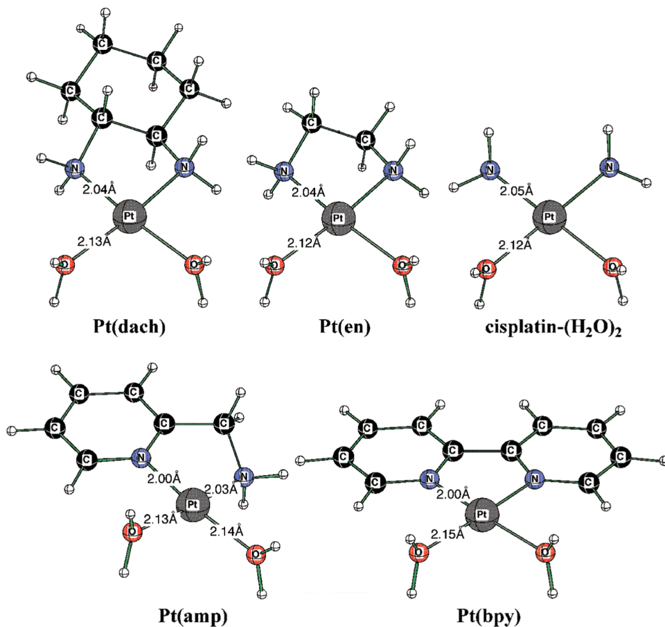
Scheme 4. Model Pt(II) complexes.
